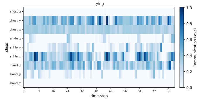
(b) Lying
