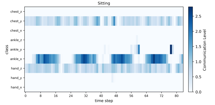
(a) Sitting
