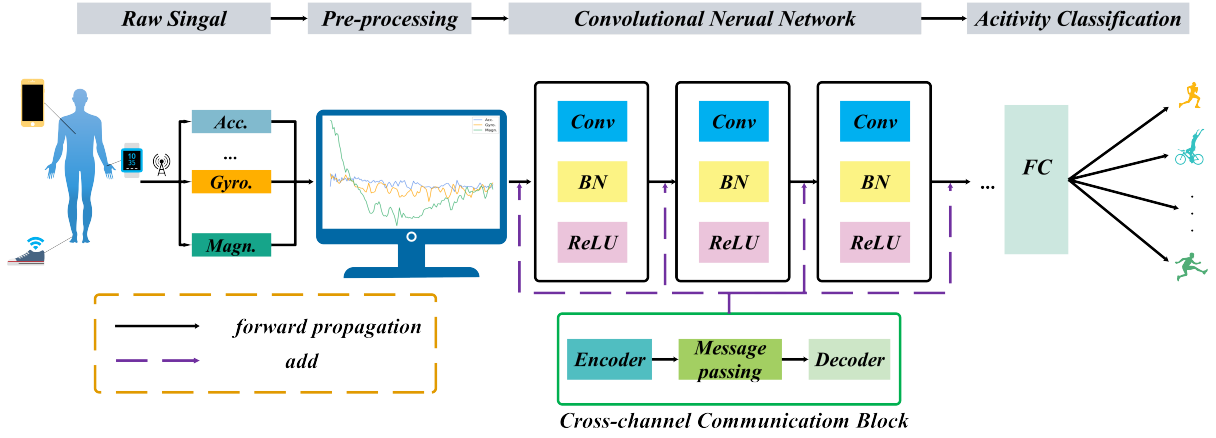
Fig. 2: The sketch map of the network with Cross-channel Communication(C3) block. The curves represent sensor time series. Sliding window is used to generate sensor examples.
