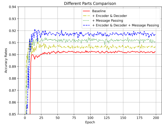
Fig. 10: Accuracy improvement caused by different parts within C3 block
