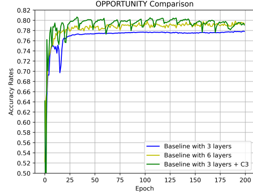
Fig. 4: Test accuracies with different models on OPPORTUNITY
