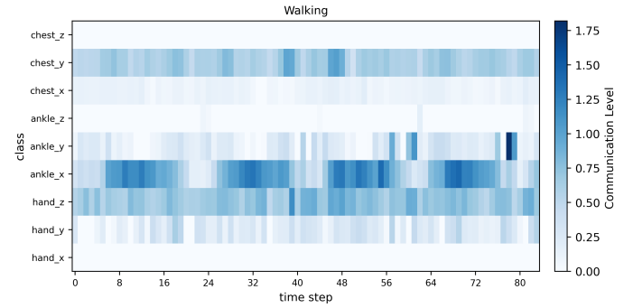
(c) Walking
