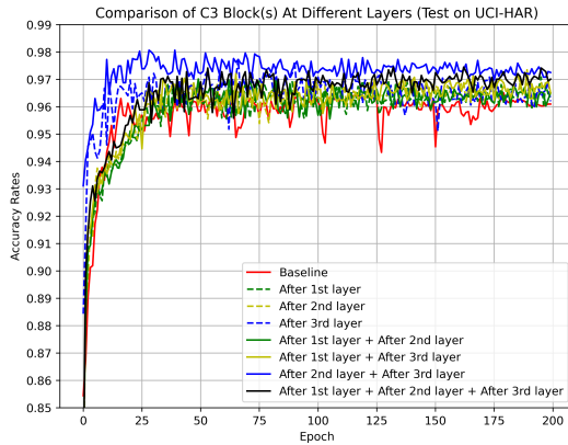
(b) UCI-HAR
