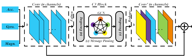
Fig. 1: The overview of C3 block
