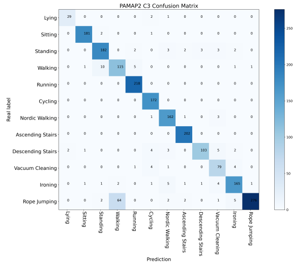
(b) 3-layer CNN + C3
