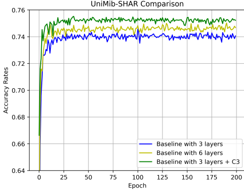
Fig. 6: Test accuracies with different models on UniMib-SHAR
