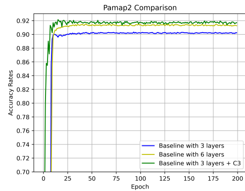
Fig. 5: Test accuracies with different models on PAMAP2
