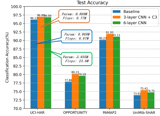
Fig. 8: Performance comparisons between shallow networks and deep networks
