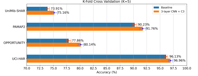
Fig. 7: K -fold cross validation ( K=5 ) on benchmark datasets
