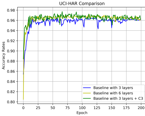
Fig. 3: Test accuracies with different models on UCI-HAR
